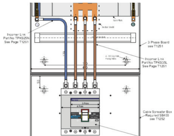
3/4 Pole 200A to 250A MCCB
