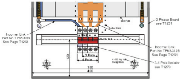
3/4 Pole Isolator 100A to 125A
