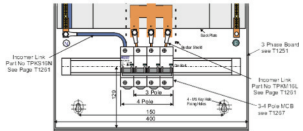
3/4 Pole MCB
