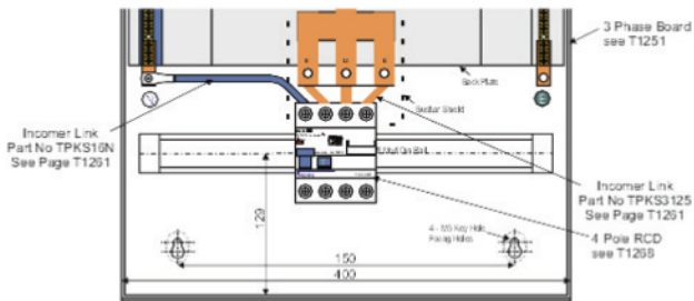
4 Pole RCD
