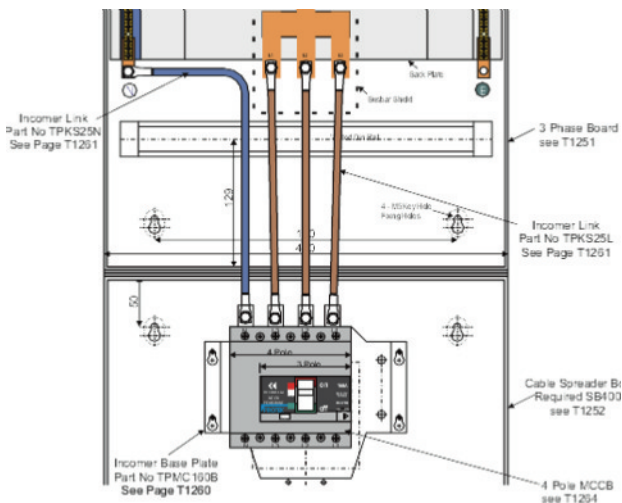
3/4 Pole 63A to 160A MCCB
